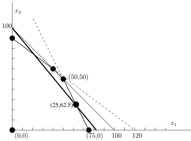
Figure 2.2 Graphical interpretation of the dual simplex iteration
